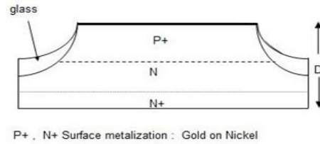
P+ , N+ Surface metalization : Gold on Nickel
